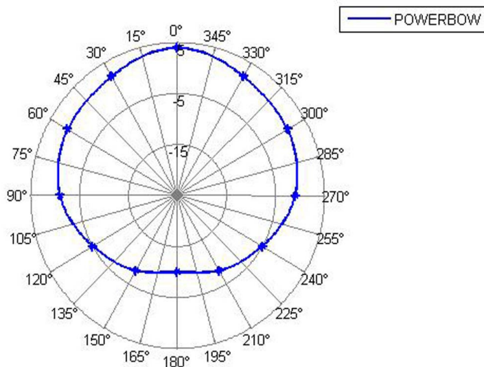
Azimuthal power pattern. Typical dBi values across passband when mounted flat on drywall
