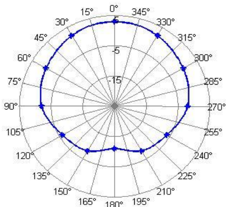
Azimuthal power pattern. DBi values when Internally Mounted at 915MHz
